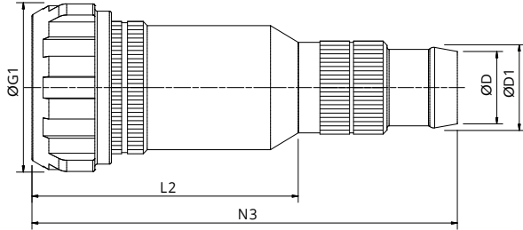
Backshell class SP
