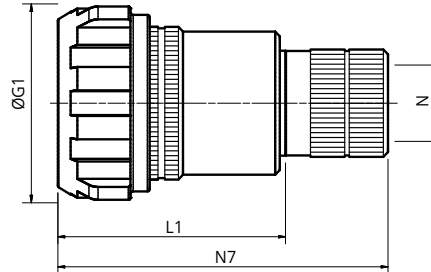
Backshell class RPM
