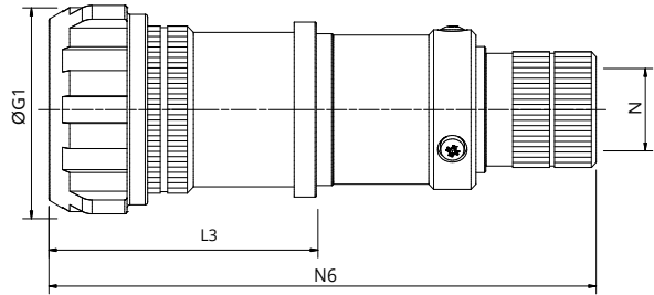
Backshell class RLM
