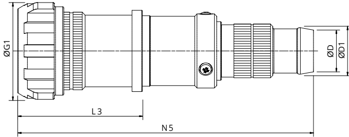
Backshell class RLP
