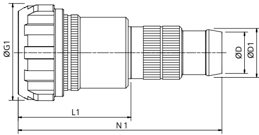
Backshell class RP
