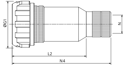
Backshell class SM
